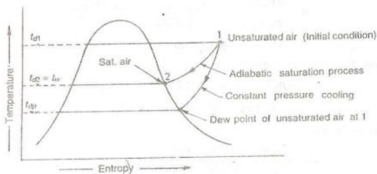
T-S Diagram for Adiabatic Saturation Process
