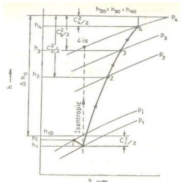
Mollier Diagram of Centrifugal Stage
