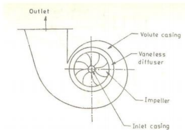
Elements of a Centrifugal Compressor
