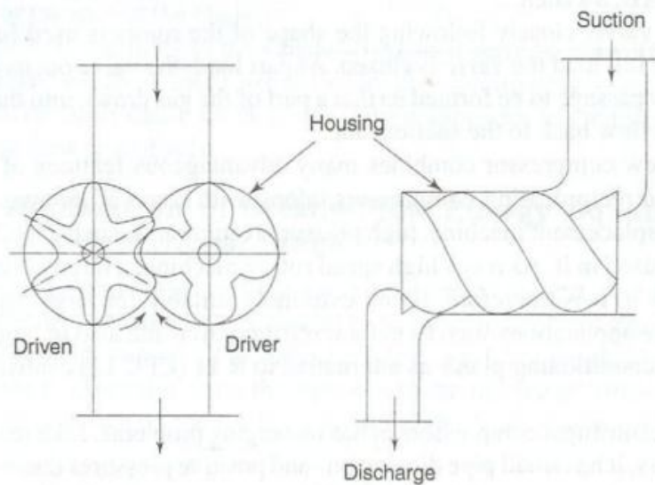
Sectional and Side Views of a Screw Compressor
